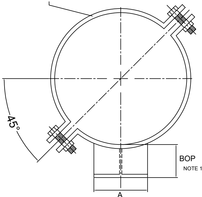
Fig 212 PIPE CLAMP
