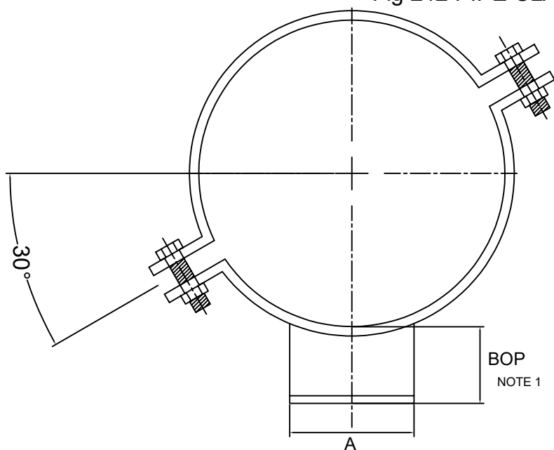
Fig 212 PIPE CLAMP
