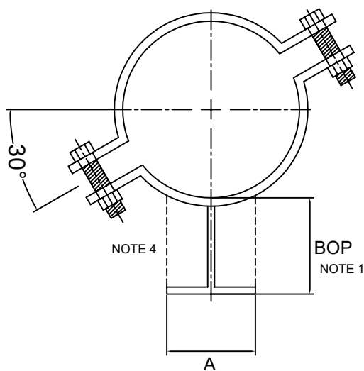
Fig 212 PIPE CLAMP
